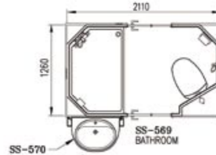
SS-570 (WITH VANITY UNIT) SS-569 BATHROOM
