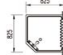
SS-132/2 SHOWER (ALTERNATIVE SIZE 800x775)
