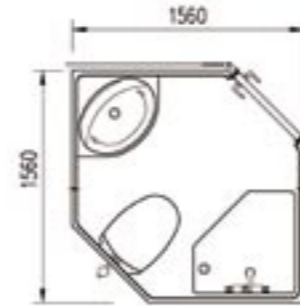
SS-119/1 BATHROOM (ALTERNATIVE SIZE 1500x1500)
