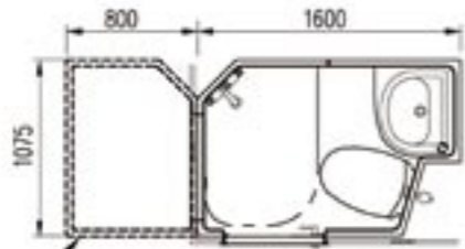
ALTERNATIVE WITH SEPARATE SHOWER SS-248/1 BATHROOM
