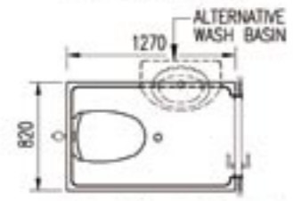
SS-112/1 EUROPEAN W.C.
